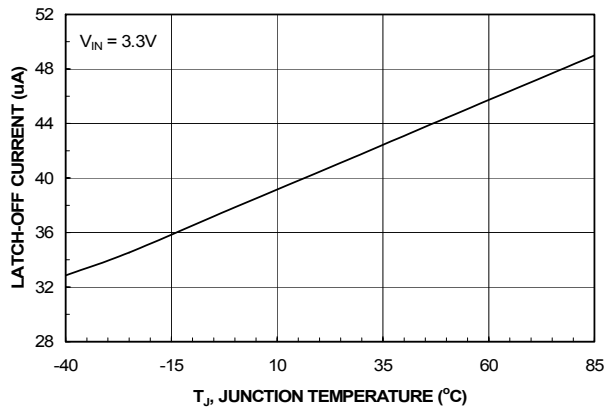
Figure 5. I_{LATC/OFF} vs. Temperature
