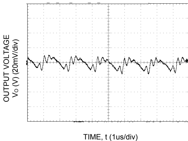
Figure 41. Typical output ripple and noise (C O =22μF ceramic, V IN = 12V, I o = I o,max , ).
