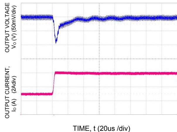
Figure 18. Transient Response to Dynamic Load Change from 50% to 100% at 12V in , C out = 2x47μF, C Tune =2200pF, R Tune =261
