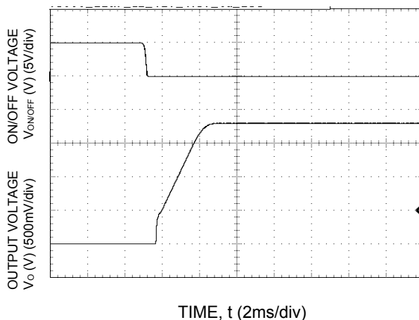
Figure 37. Typical Start-up Using On/Off Voltage (I o = I o,max ).
