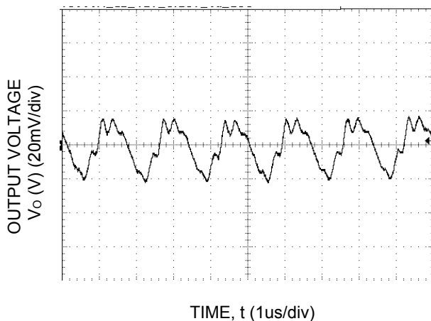
Figure 23. Typical output ripple and noise (C O =22μF ceramic, V IN = 12V, I o = I o,max , ).
