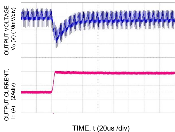
Figure 42. Transient Response to Dynamic Load Change from 50% to 100% at 12V IN , C out =1x47μF + 2x330μF, C Tune =12nF, R Tune =178
