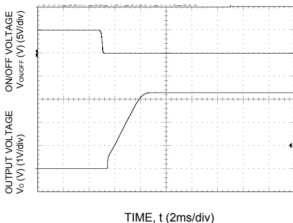
Figure 25. Typical Start-up Using On/Off Voltage (I o = I o,max ).
