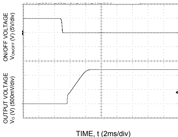
Figure 43. Typical Start-up Using On/Off Voltage (I o = I o,max ).
