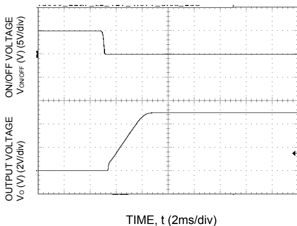
Figure 19. Typical Start-up Using On/Off Voltage (I o = I o,max ).
