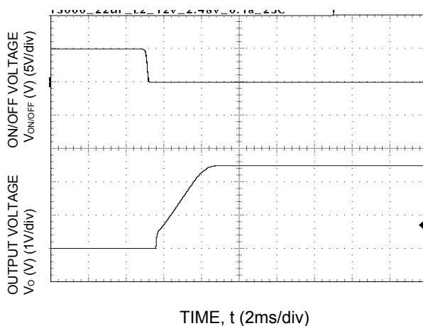
Figure 31. Typical Start-up Using On/Off Voltage (I o = I o,max ).
