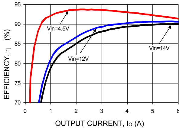
Figure 27. Converter Efficiency versus Output Current.
