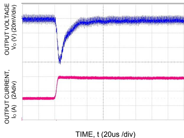
Figure 24 Transient Response to Dynamic Load Change from 50% to 100% at 12V in , C out = 3x47μF, C Tune =3300pF, R Tune =178
