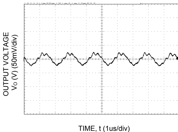
Figure 17. Typical output ripple and noise (C O =22μF ceramic, V IN = 12V, I o = I o,max , ).
