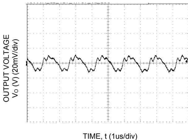
Figure 35. Typical output ripple and noise (C O =22μF ceramic, V IN = 12V, I o = I o,max , ).
