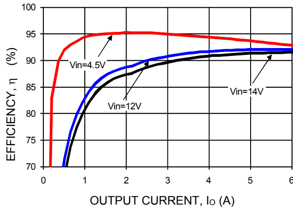
Figure 21. Converter Efficiency versus Output Current.
