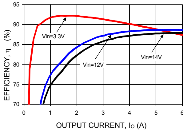
Figure 33. Converter Efficiency versus Output Current.
