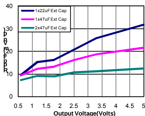
Fig-2: Output ripple voltage for various output voltages with external 1x22uF, 1x47uF or 2x47uF ceramic capacitors at the output (6A load). Input voltage is 12V.
