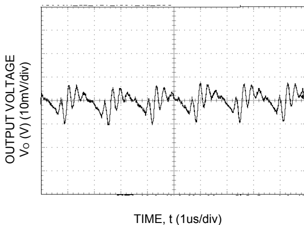
Figure 47. Typical output ripple and noise (C O =22μF ceramic, V IN = 12V, I o = I o,max ).
