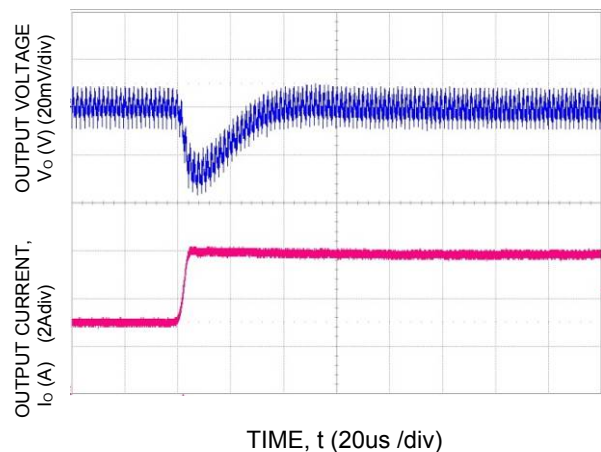
Figure 36. Transient Response to Dynamic Load Change from 50% to 100% at 12V in , C out = 1x47μF + 1x330μF, C Tune =4700pF, R Tune =178
