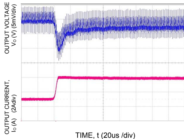
Figure 48. Transient Response to Dynamic Load Change from 50% to 100% at 12V in , C out =1x47μF + 4x330μF, C Tune =33nF, R Tune =178
