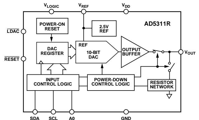
Figure 2. AD5311R
