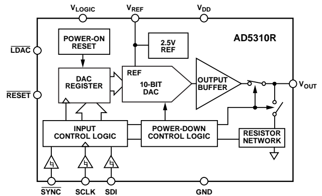
Figure 1. AD5310R
