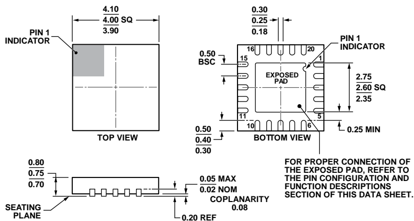
Figure 52. 20-Lead Lead Frame Chip Scale Package [LFCSF] 4 mm × 4 mm Body and 0.75 mm Package Height (CP-20-8)
