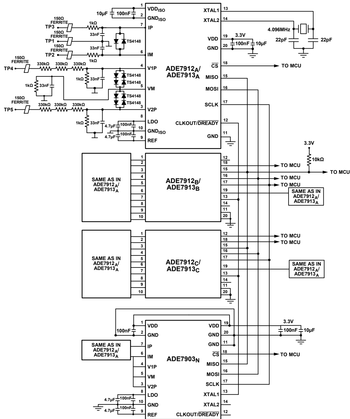
Figure 18. Test Circuit
