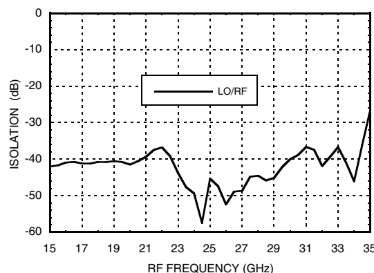
LO/RF Isolation
