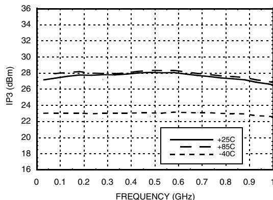
IP3 vs. Temperature @ 3V
