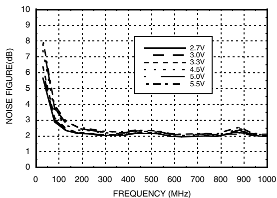
Noise Figure vs. Supply Voltage
