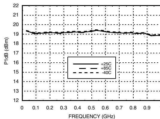
P1dB vs. Temperature @ 5V
