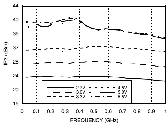
IP3 vs. Supply Voltage
