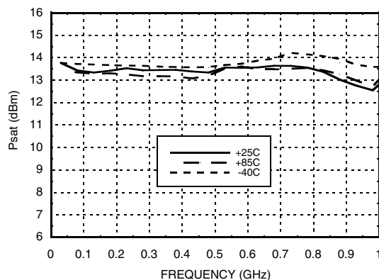
Psat vs. Temperature @ 3V
