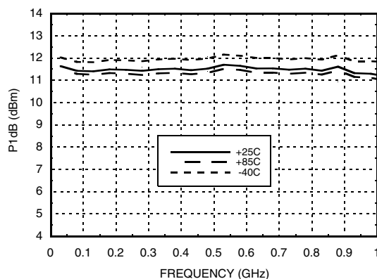
P1dB vs. Temperature @ 3V
