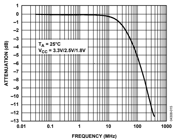
Figure 15. Bandwidth
