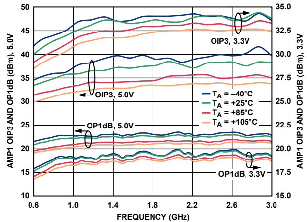
Figure 6. AMP1 OIP3 at P_{OUT} = 0\text{ dBm/Tone} and OP1dB vs. Frequency by Temperature
