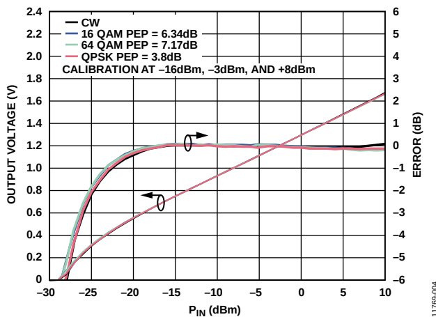
Figure 4. Error from CW Linear Reference vs. Input Level and Signal Modulation (QPSK, 16 QAM, 64 QAM), Frequency = 900 MHz, C_{RMS} = 1 \mu F
