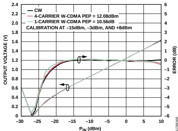
Figure 5. Error from CW Linear Reference vs. Input Level and Signal Modulation (One-Carrier W-CDMA, Four-Carrier W-CDMA), Frequency = 2.14 GHz, C_{RMS} = 1 \mu F
