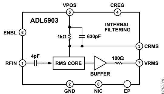
Figure 39. Simplified Architecture
