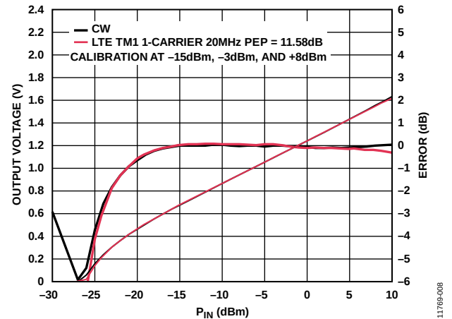
Figure 8. Error from CW Linear Reference vs. Input Level and Signal Modulation (LTE TM1 One-Carrier, 20 MHz), Frequency = 2.14 GHz, C_{RMS} = 1 \mu F
