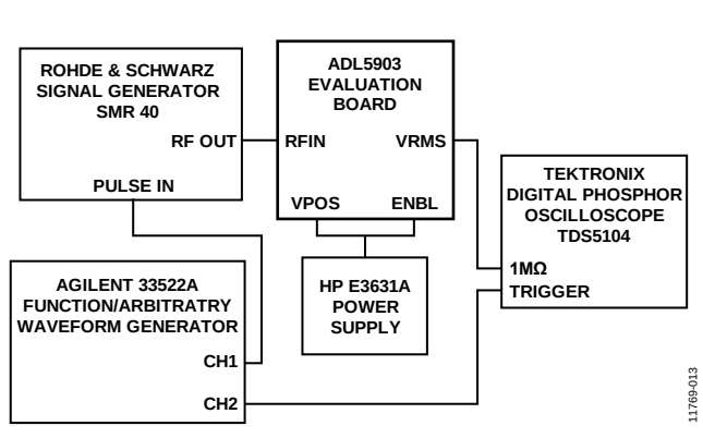
Figure 36. Hardware Configuration for Output Response to RF Burst Input Measurements
