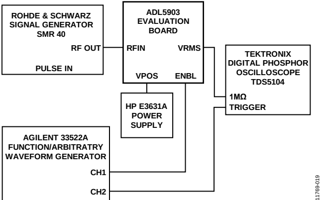
Figure 38. Hardware Configuration for Output Response to ENBL Pin Gating Measurements
