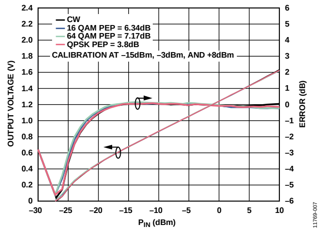
Figure 7. Error from CW Linear Reference vs. Input Level and Signal Modulation (QPSK, 16 QAM, 64 QAM), Frequency = 2.14 GHz, C_{RMS} = 1 \mu F
