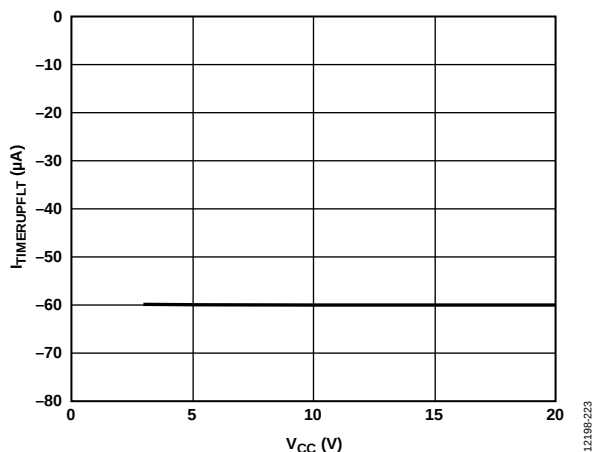
Figure 20. TIMER Pull-Up Current OC Fault ( I_{T\text{IMERUPELT}} ) vs. V_{CC}
