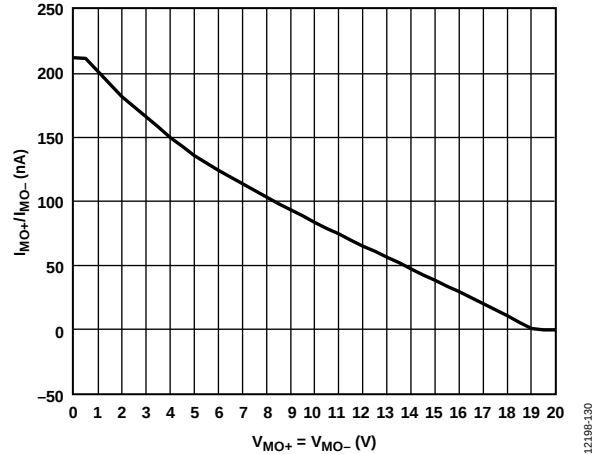
Figure 40. I_{MO+}/I_{MO-} vs. V_{MO+}/V_{MO-} with V_{CC} = 20\text{ V}
