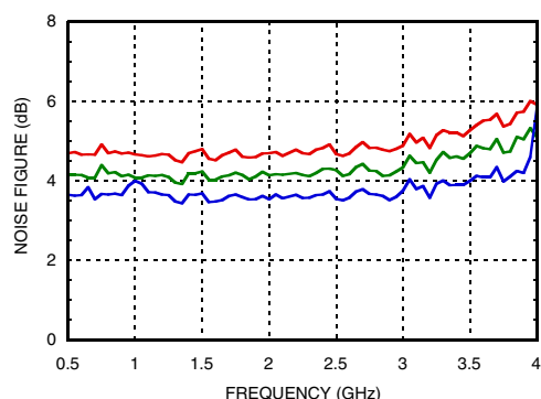
Noise Figure vs. Frequency [1]
