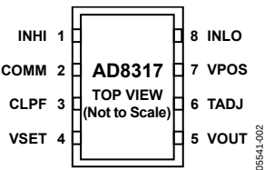
Figure 2. Pin Configuration
