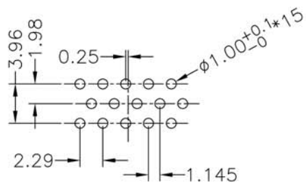
15 Pin Female Connector PCB Pin Layout Scale 2:1
