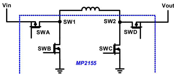
Figure 2—Buck-Boost Switch Topology
