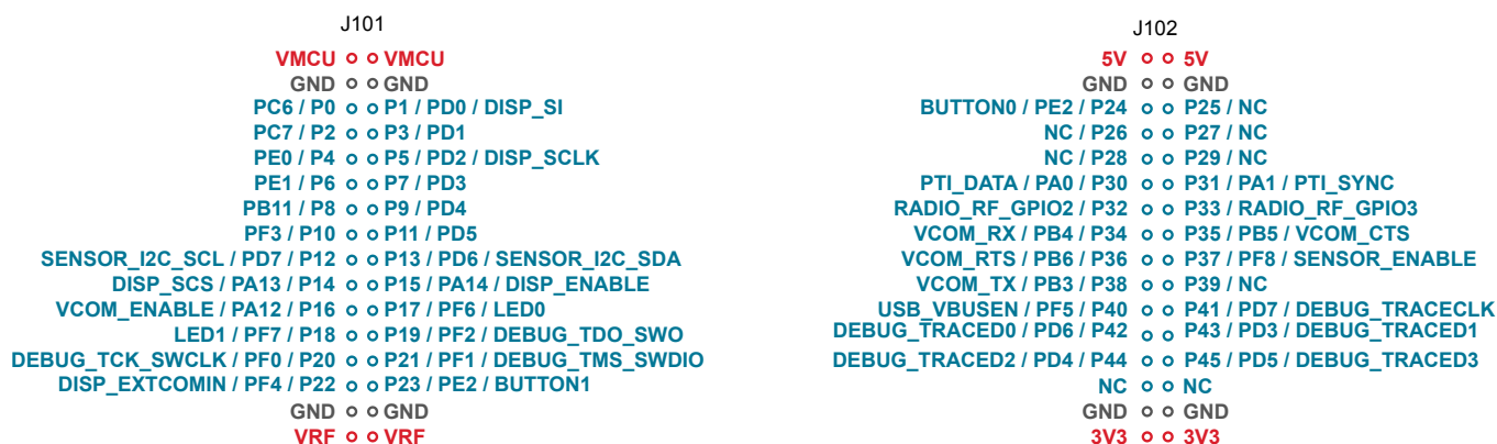
Figure 4.2. Radio Board Pin Mapping on Breakout Pads
