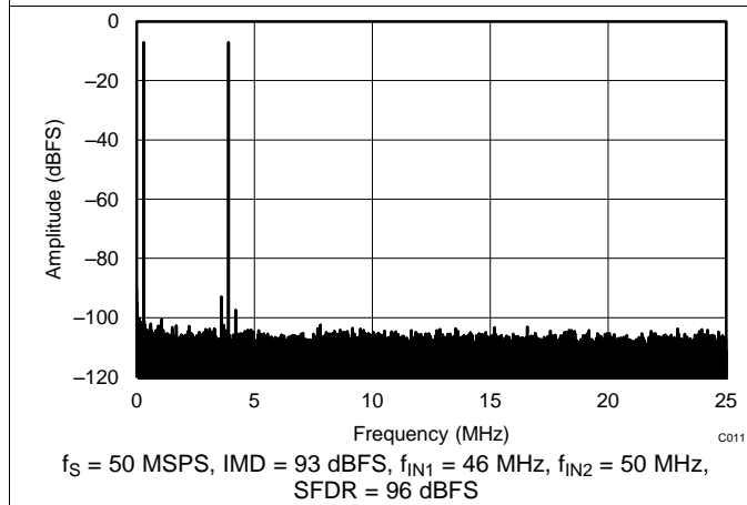
Figure 110. FFT for Two-Tone Input Signal (-7dBFS at 46 MHz and 50 MHz)
