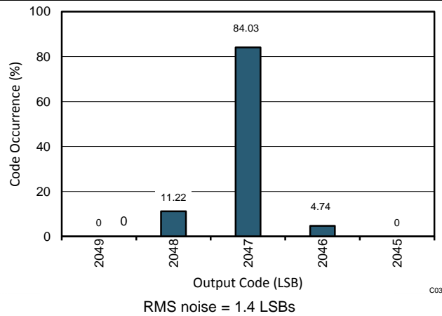
Figure 99. Idle Channel Histogram
