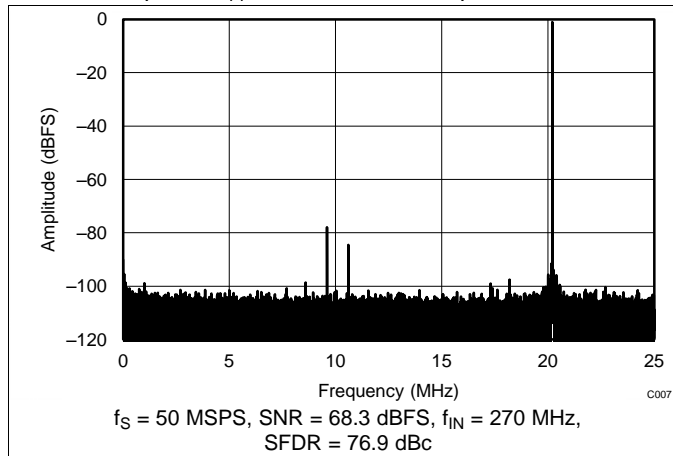
Figure 106. FFT for 270-MHz Input Signal (Dither On)
