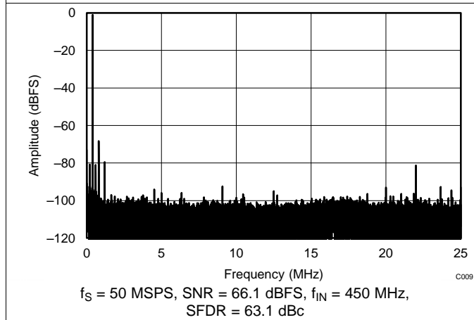
Figure 108. FFT for 450-MHz Input Signal (Dither On)
