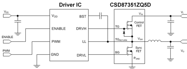
TYPICAL CIRCUIT
