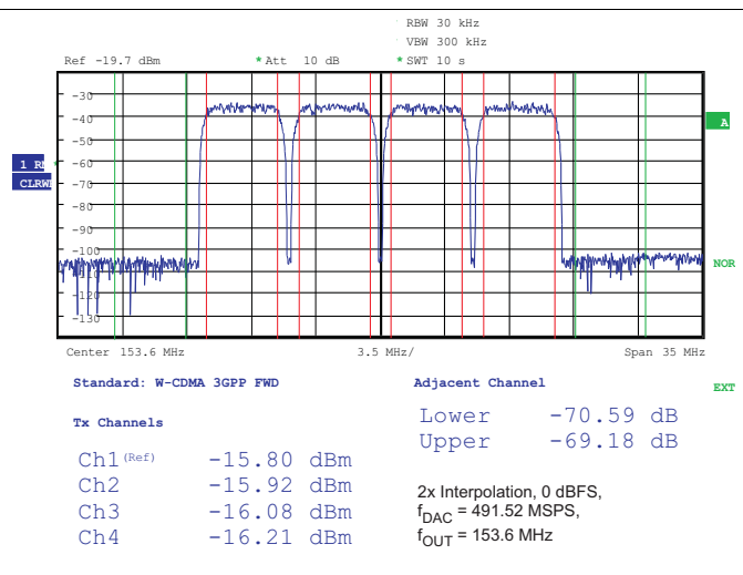
Figure 88. Four Carrier W-CDMA Test Model 1, f_{OUT} = 153.6 \text{ MHz}
