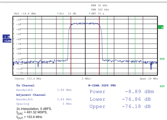
Figure 86. Single Carrier W-CDMA Test Model 1, f_{OUT} = 153.6 \text{ MHz}
