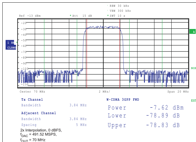
Figure 85. Single Carrier W-CDMA Test Model 1, f_{OUT} = 70 \text{ MHz}
