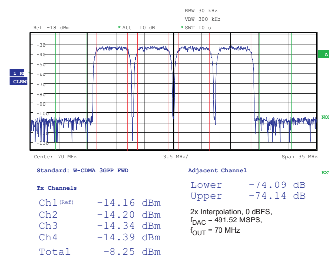
Figure 87. Four Carrier W-CDMA Test Model 1, f_{OUT} = 70 \text{ MHz}
