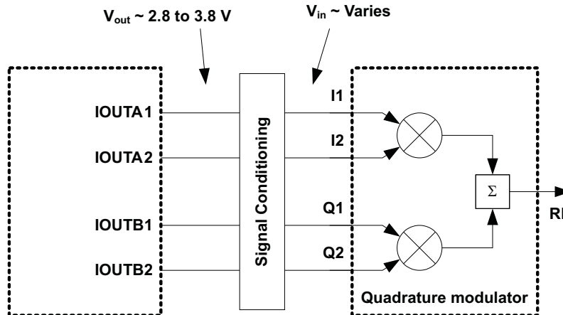
Figure 80. DAC to Analog Quadrature Modulator Interface
