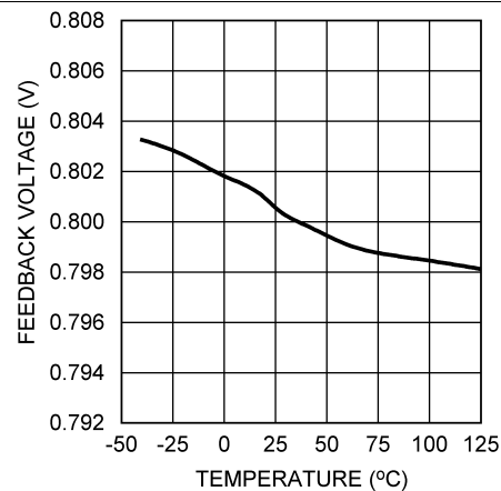
Figure 12. Feedback Pin Voltage vs Temperature
