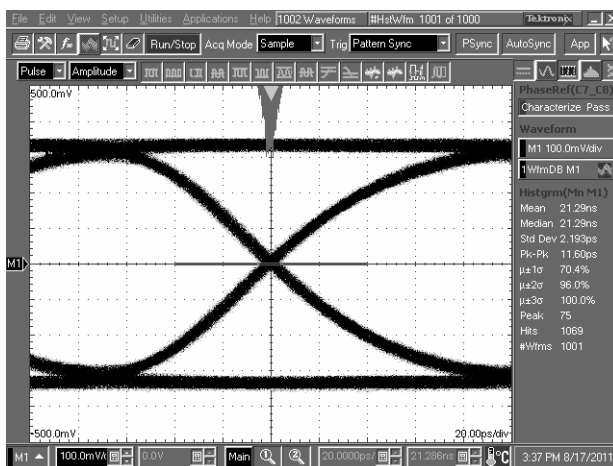
Figure 17. De-Emphasis Performance with 10" of 4 mil FR4 using DE setting 0x02
