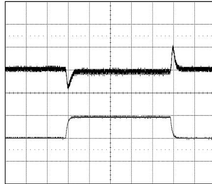
Conditions: Input Voltage = 24 VDC Output Current = 5 to 10 A Bandwidth Limit = 20 MHz Traces: Bottom Trace: Output current A/div = 5 A Top Trace: Output voltage response V/div = 100 mV Horizontal Resolution = 200 \mu s/div
