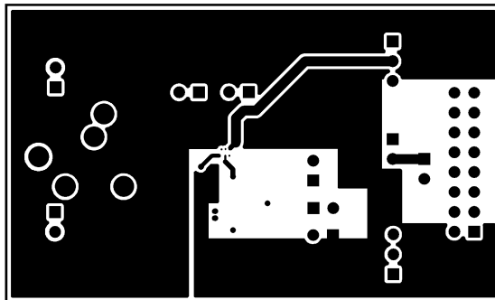
Figure 40. Internal Layer 2
