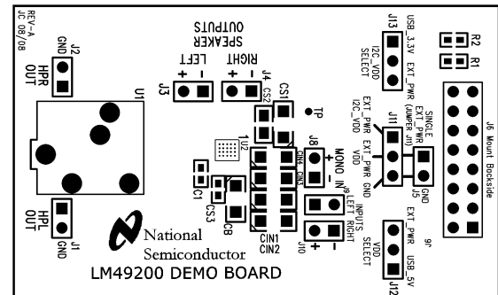
Figure 37. Silk Screen
