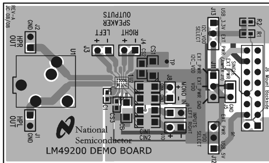
Figure 36. Composite View
