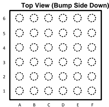
Figure 3. 36 - Bump DSBGA Package See Package Number YPG0036LVA
