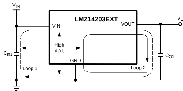
Figure 35. Critical Current Loops to Minimize
