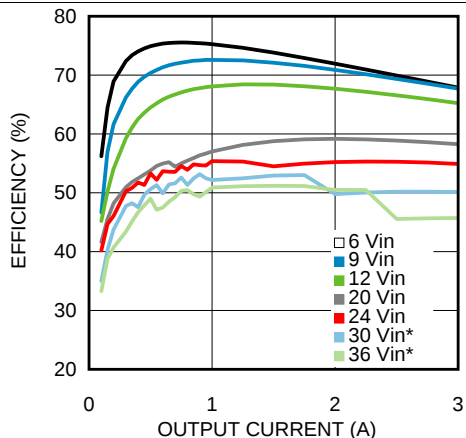
Figure 31. Efficiency 1.2-V Output at 85°C Ambient
