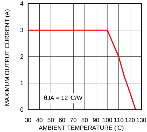
Figure 38. Thermal Derating
