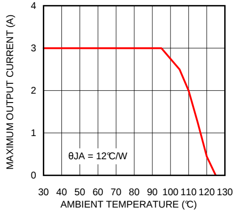
Figure 37. Thermal Derating
