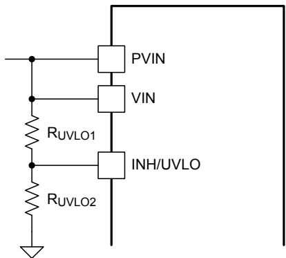
Figure 41. Adjustable VIN and PVIN Undervoltage Lockout
