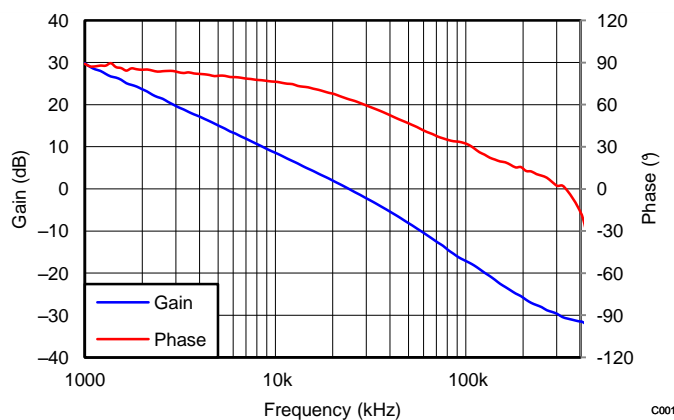
Figure 16. V OUT = 1.8 V, I OUT = 7 A, C OUT = 200 \mu F ceramic, f SW = 500 kHz
