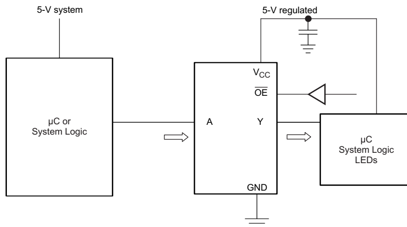
Figure 5. Typical Application Schematic
