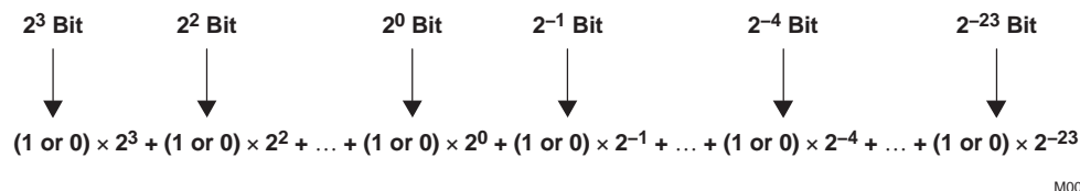
Figure 2-5. Conversion Weighting Factors—5.23 Format to Floating Point
