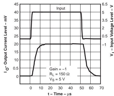
TURN-ON AND TURN-OFF TIME vs DELAY TIME
