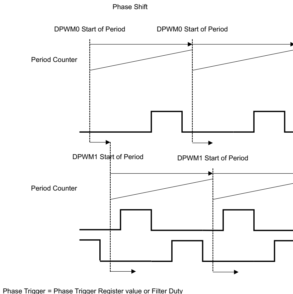
Figure 6-23. Phase Shifting
