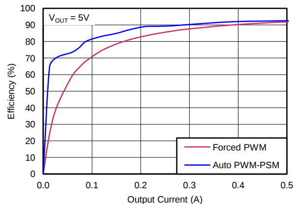
Figure 10. 5-V Efficiency, Light Load V_{IN} = 12\text{ V} , V_{OUT} = 5\text{ V}
