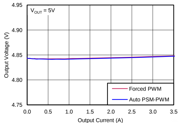
Figure 14. 5-V Load Regulation V_{IN} = 12\text{ V} , V_{OUT} = 5\text{ V}
