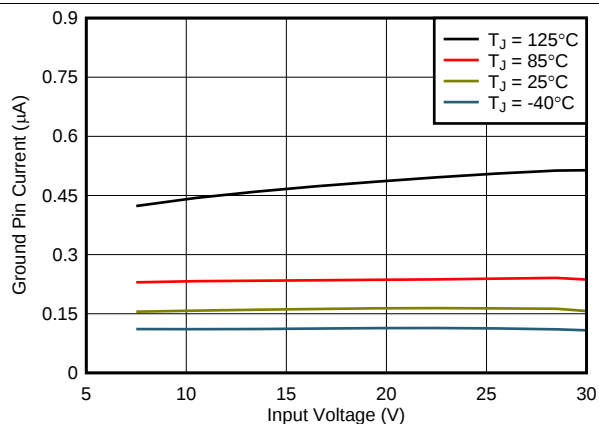
Figure 21. 1.2-V Shutdown Current vs V_{IN} and Temperature
