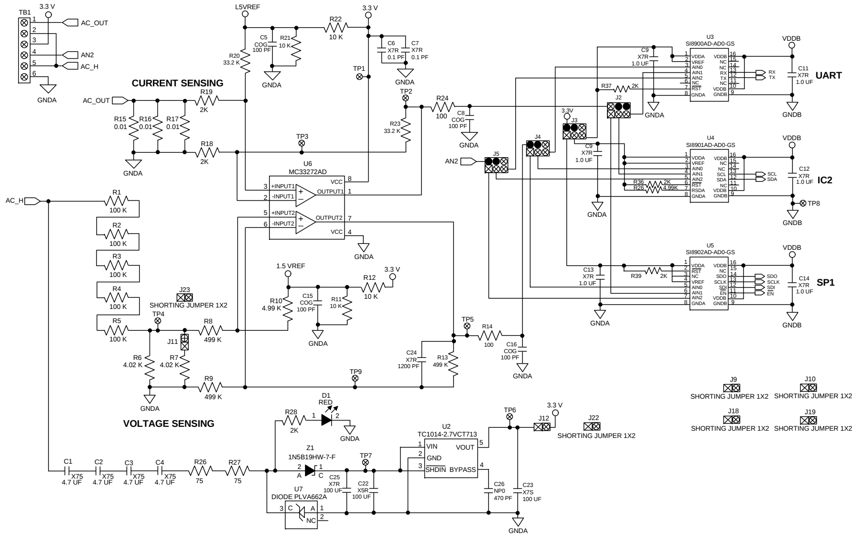
Figure 9. Measurement Circuits
