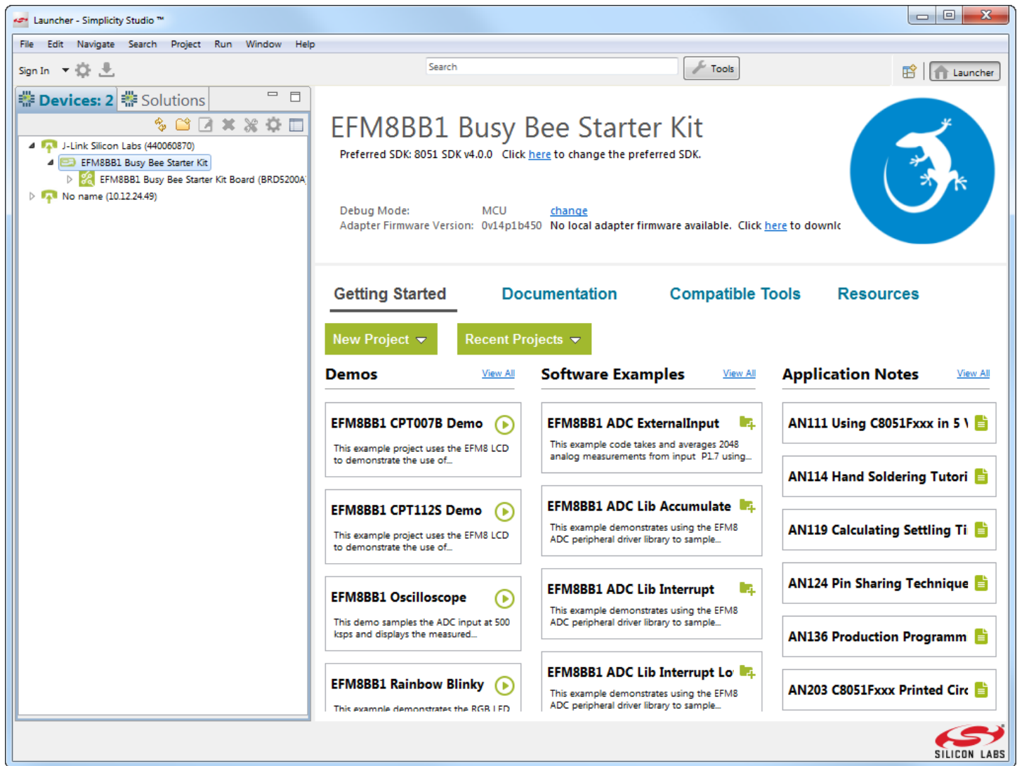
Figure 7.1. Simplicity Studio
