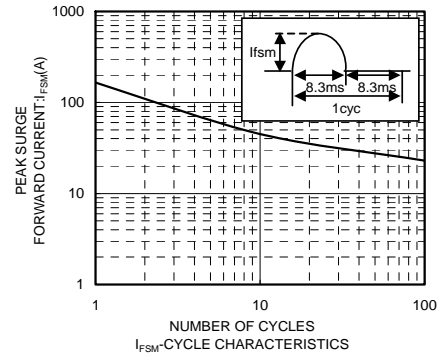
I_{FSM} -C CYCLE CHARACTERISTICS
