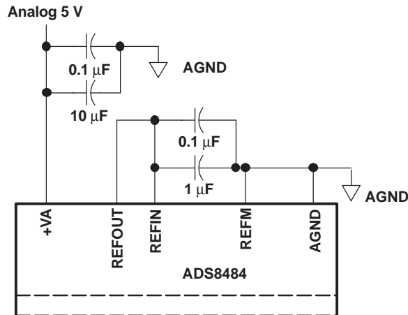
Figure 37. ADS8484 Using Internal Reference
