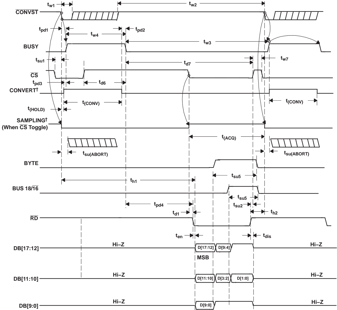
Figure 31. Timing for Conversion and Acquisition Cycles With CS and RD Toggling
