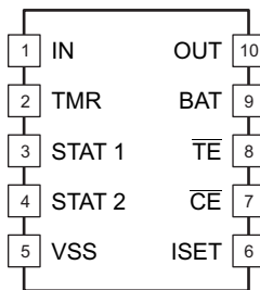
bq24087 DRC Package 10-Pin VSON Top View
