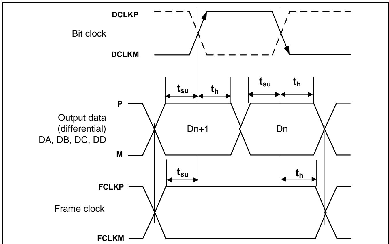
Figure 2. LVDS Timings
