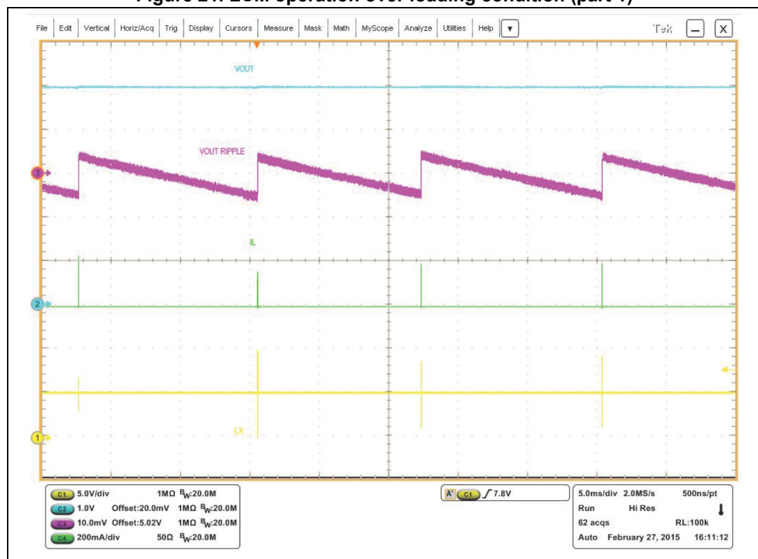
Figure 21. LCM operation over loading condition (part 1)
