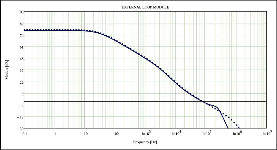
Figure 40. Magnitude plot for Example 2
