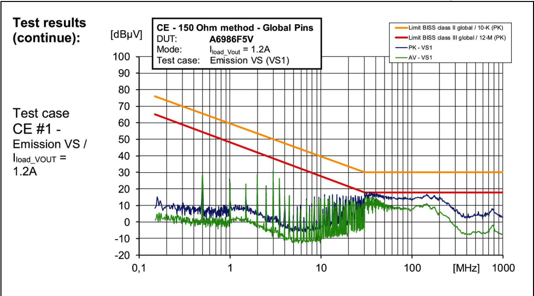
Figure 65. CE 150R at VS1 test point (see Figure 64 ) at 80% I LOAD
