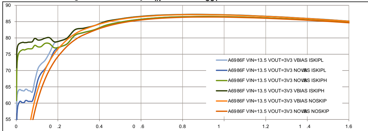
Figure 57. Efficiency curves: V_{IN} = 13.5\text{ V} - V_{OUT} = 3.3\text{ V} - f_{sw} = 500\text{ kHz} (log scale)
