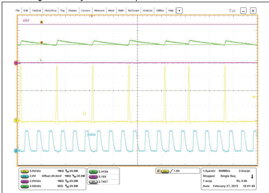
Figure 29. Valley current sense operation in overcurrent condition
