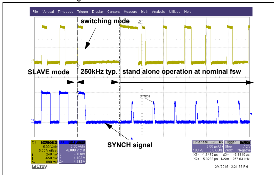
Figure 49. Slave to master mode transition
