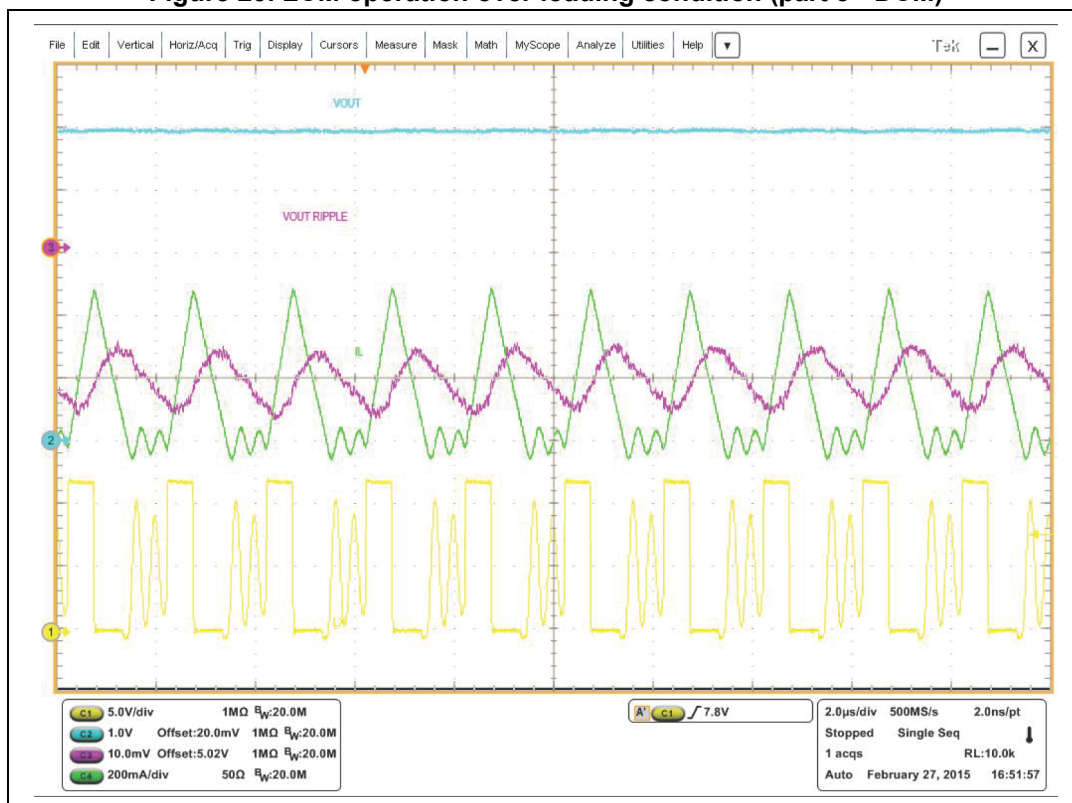
Figure 23. LCM operation over loading condition (part 3 - DCM)
