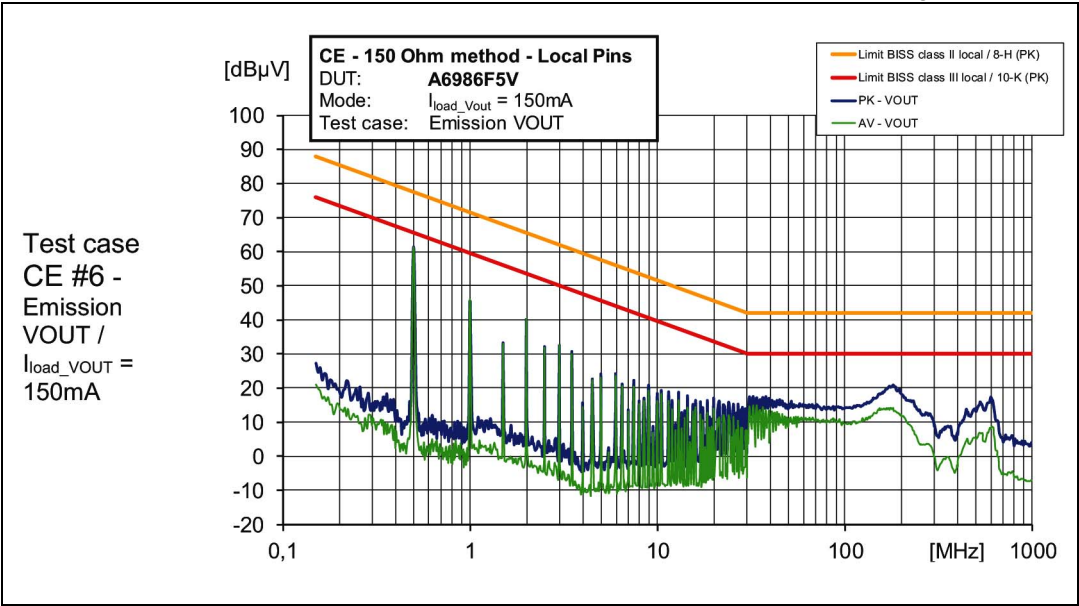
Figure 68. CE 150R at VOUT test point (see Figure 64) at 10% I LOAD
