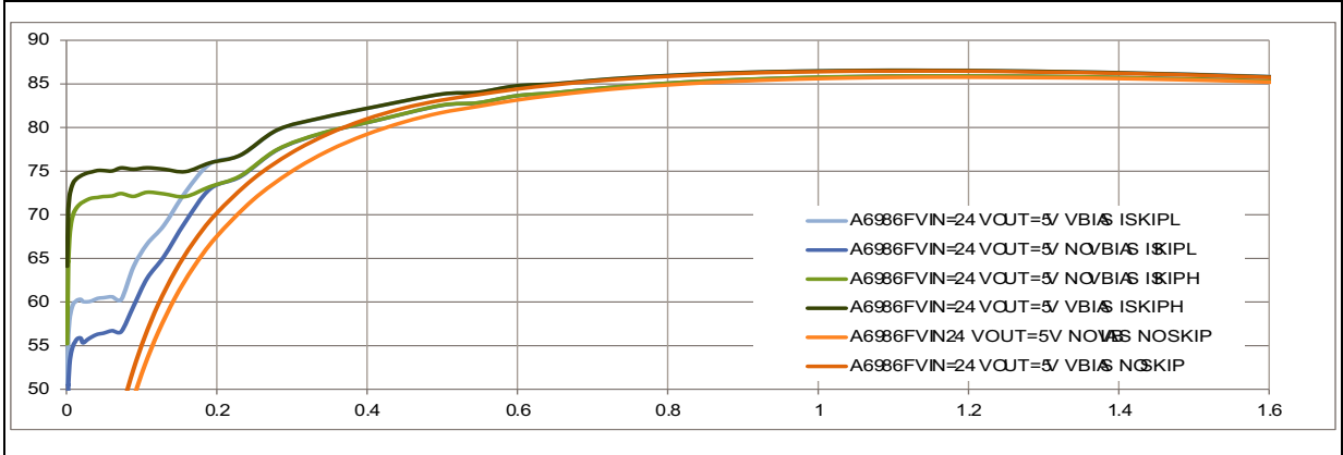
Figure 62. Efficiency curves: V_{IN} = 24\text{ V} - V_{OUT} = 5\text{ V} - f_{sw} = 500\text{ kHz}
