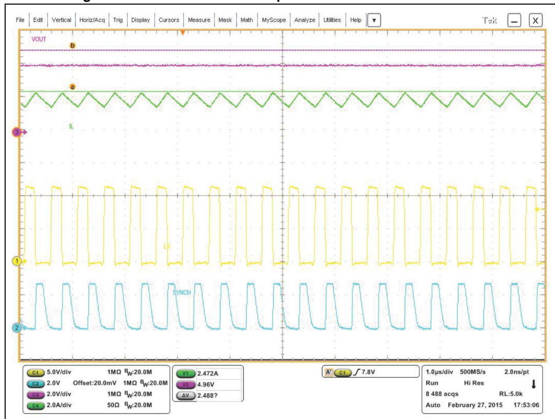
Figure 30. Peak current sense operation in overcurrent condition
