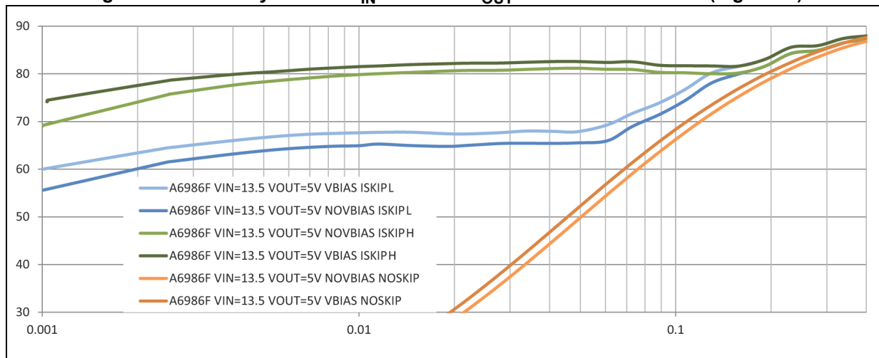
Figure 60. Efficiency curves: V_{IN} = 24\text{ V} - V_{OUT} = 3.3\text{ V} - f_{sw} = 500\text{ kHz}
