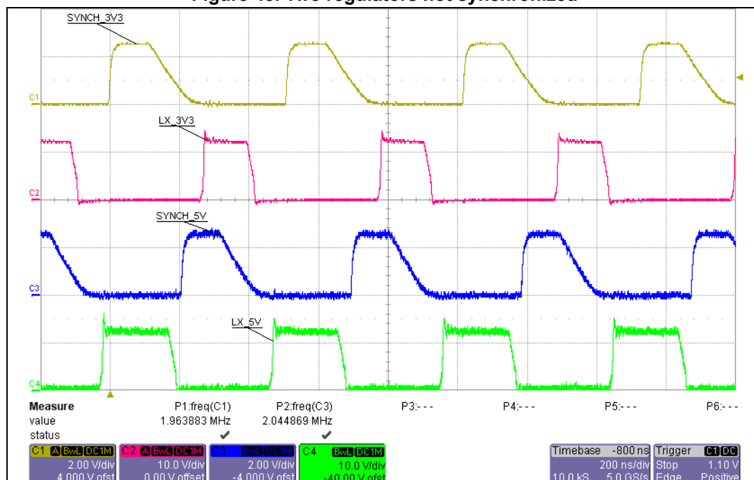
Figure 45. Two regulators not synchronized
