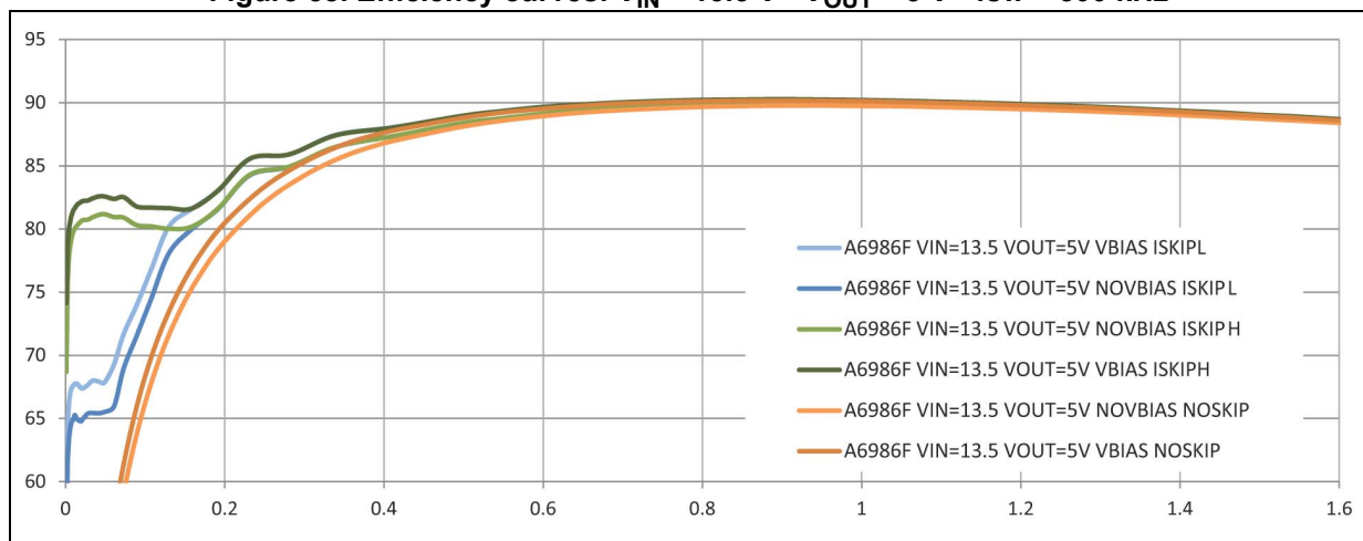
Figure 58. Efficiency curves: V_{IN} = 13.5\text{ V} - V_{OUT} = 5\text{ V} - f_{sw} = 500\text{ kHz}
