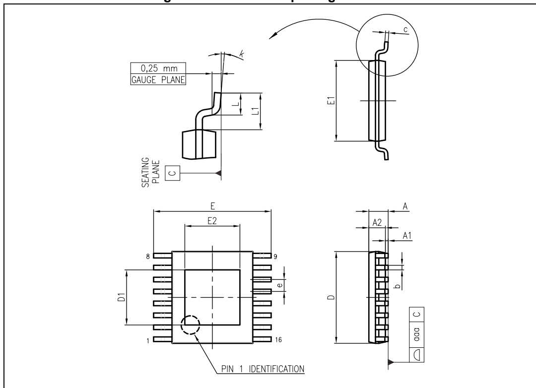
Figure 73. HTSSOP16 package outline
