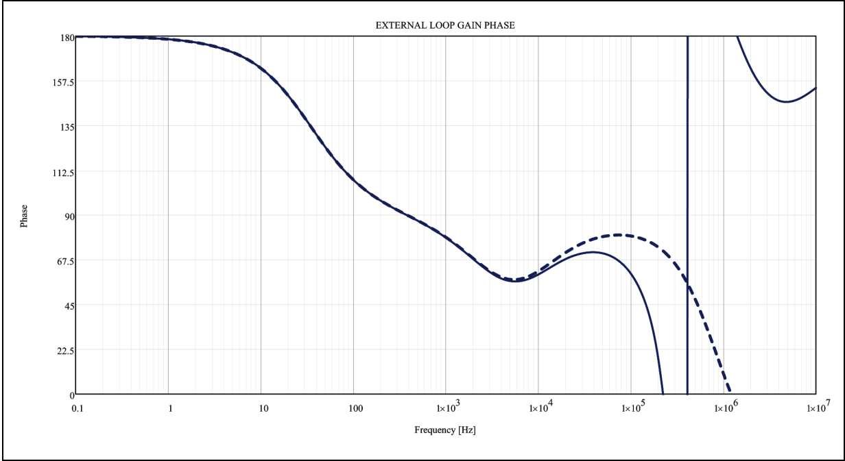
Figure 53. Phase margin Bode's plot
