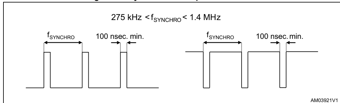
Figure 47. Synchronization pulse definition
