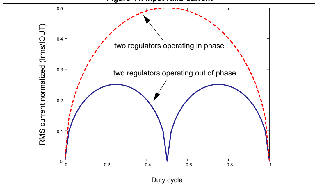
Figure 44. Input RMS current
