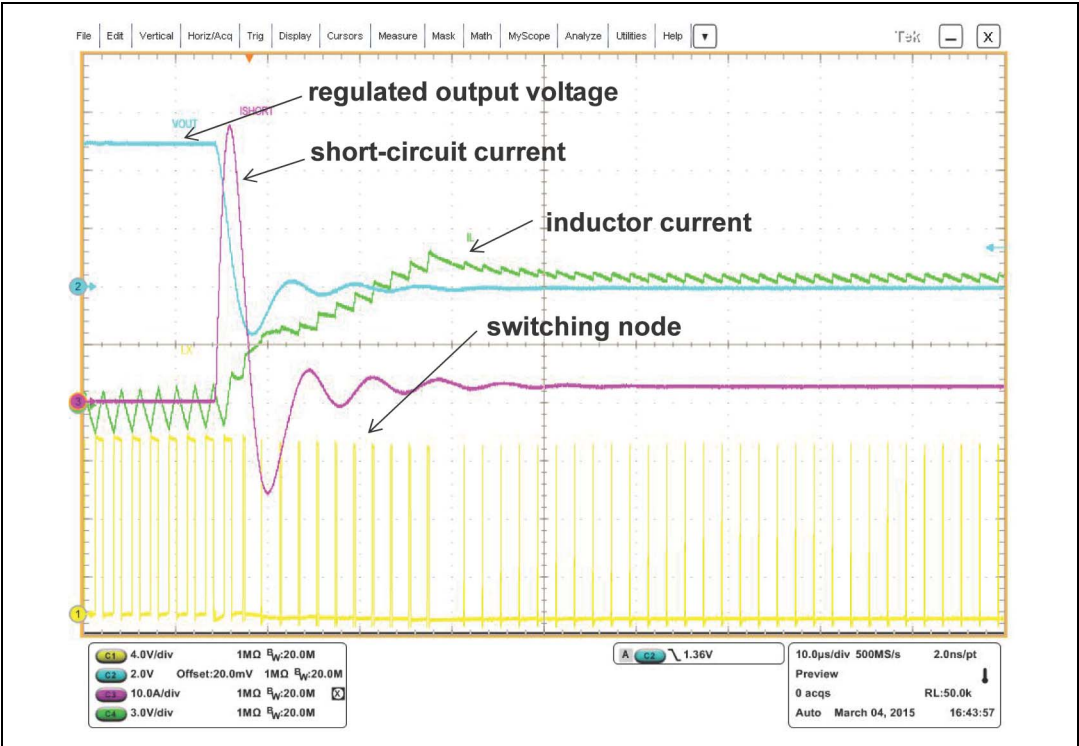
Figure 31. Output voltage oscillations during heavy short-circuit
