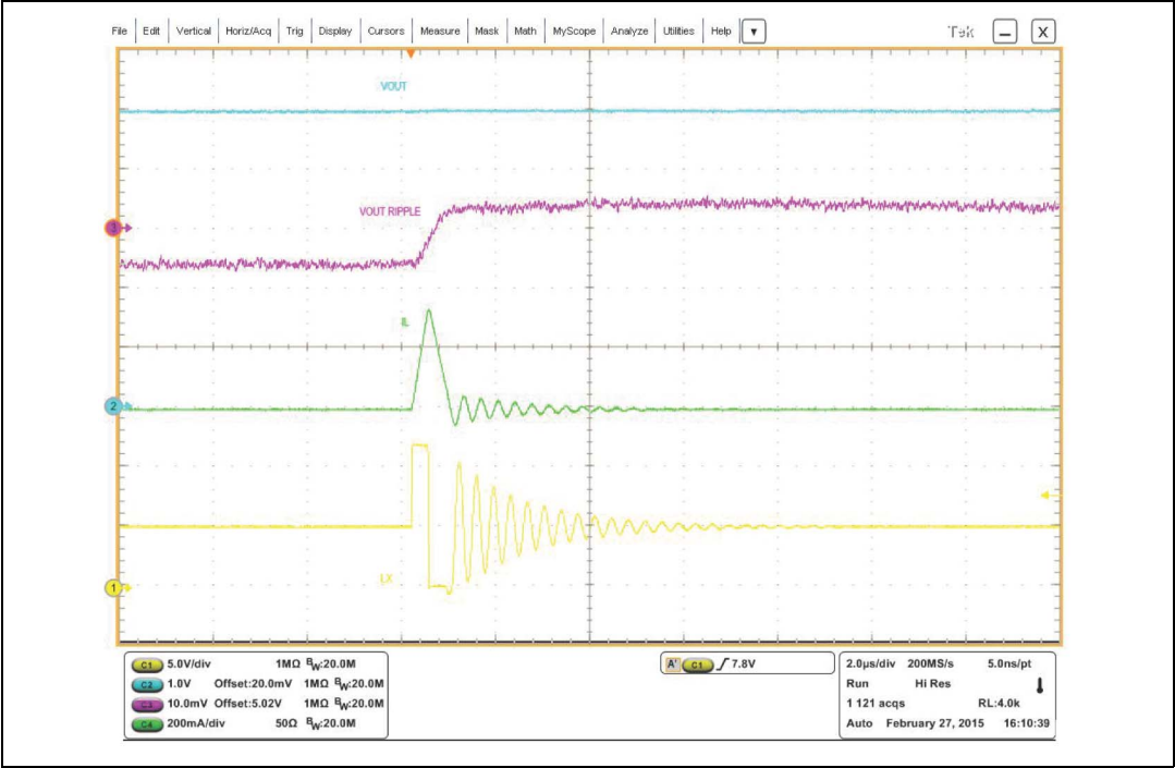
Figure 20. LCM operation with ISKIP_L = 200\text{ mA typ.} at zero load
