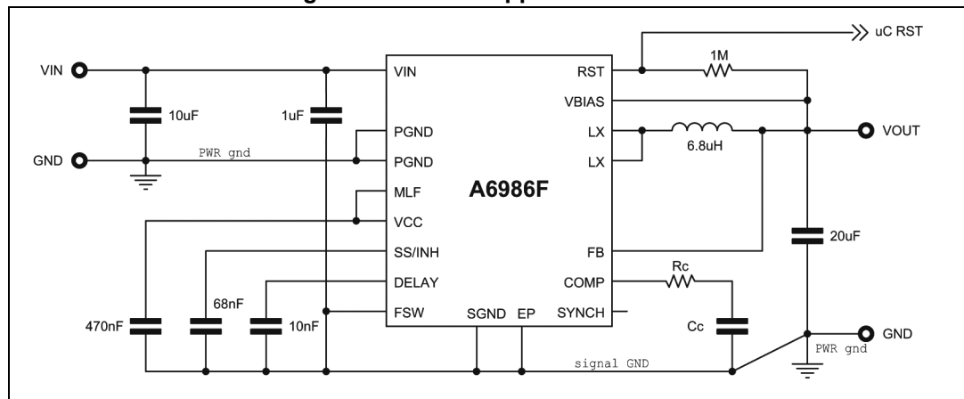
Figure 42. A6986F application circuit
