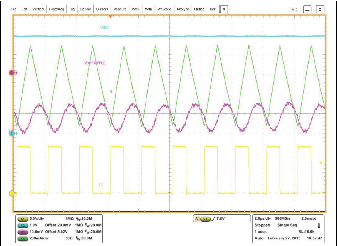
Figure 25. LCM operation over loading condition (part 5 - CCM)
