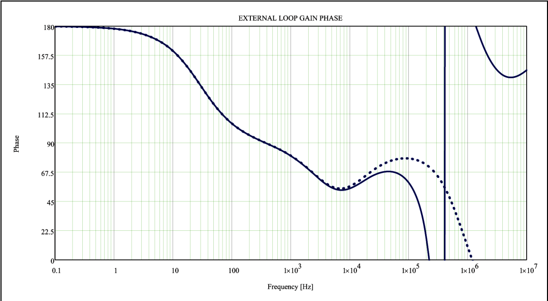
Figure 41. Phase plot for Example 2
