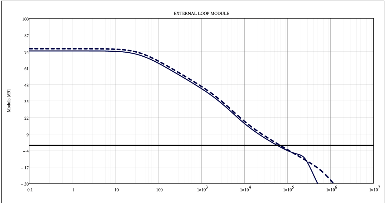
Figure 52. Magnitude Bode’s plot
