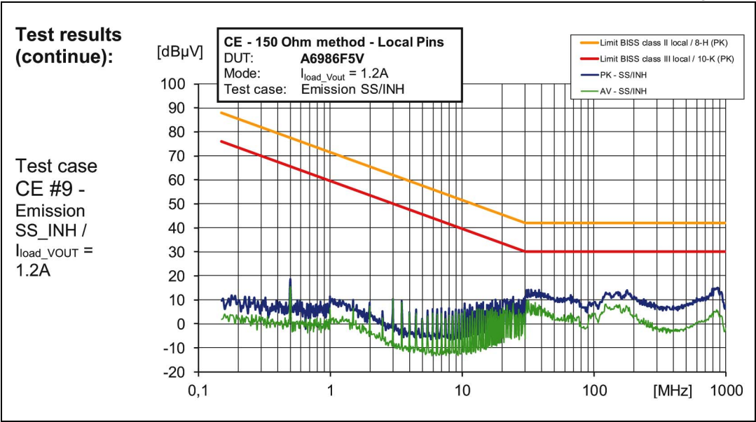
Figure 71. CE 150R at SS/INH test point (see Figure 64 on page 68 ) at 80% I LOAD
