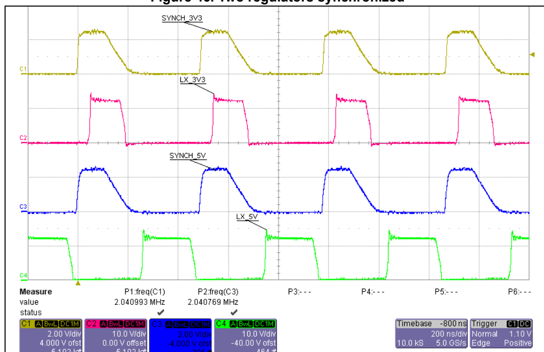
Figure 46. Two regulators synchronized
