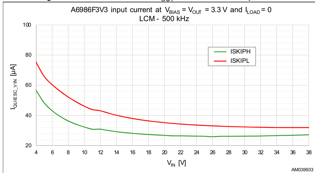
Figure 26. Quiescent current at V_{OUT} = 3.3\text{ V} and zero output load
