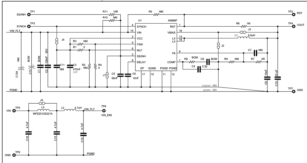
Figure 51. Evaluation board schematic
