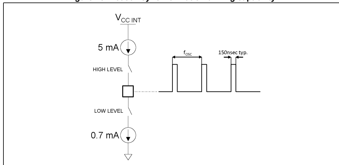
Figure 48. A6986F synchronization driving capability
