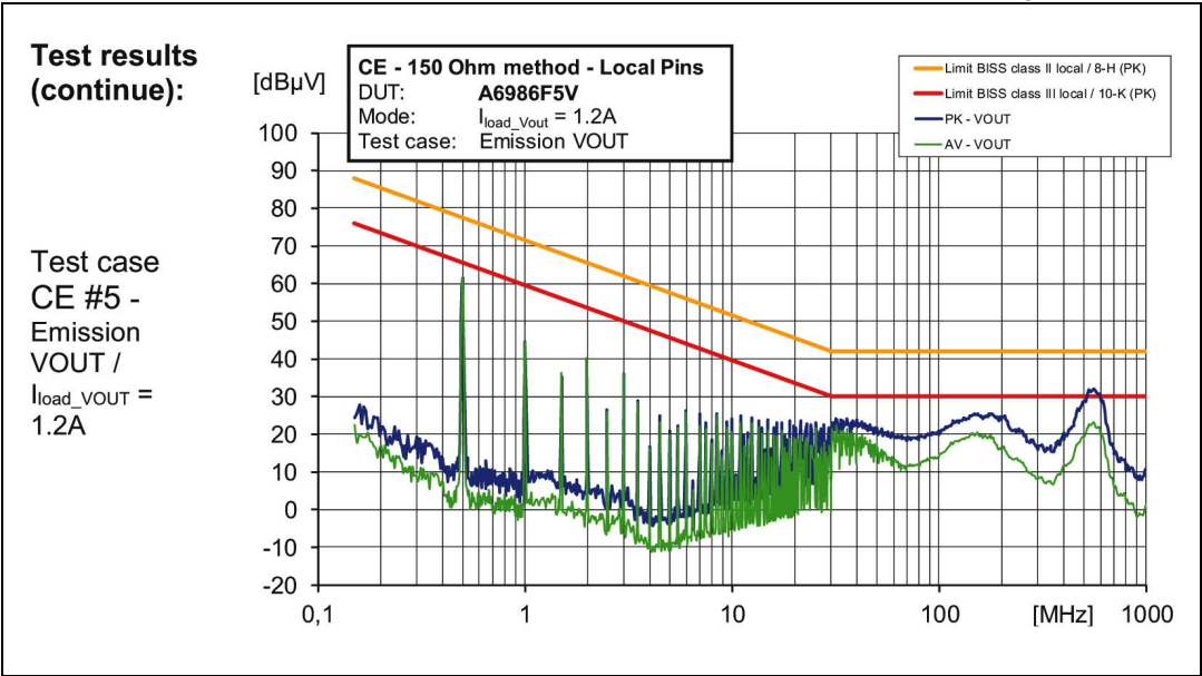
Figure 67. CE 150R at VOUT test point (see Figure 64) at 80% I LOAD
