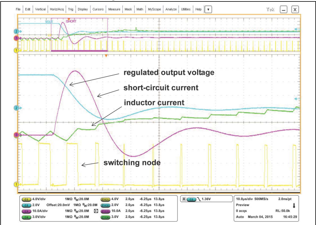
Figure 32. Zoomed waveform
