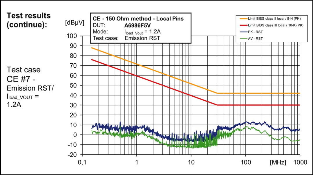
Figure 69. CE 150R at RST test point (see Figure 64 ) at 80% I LOAD
