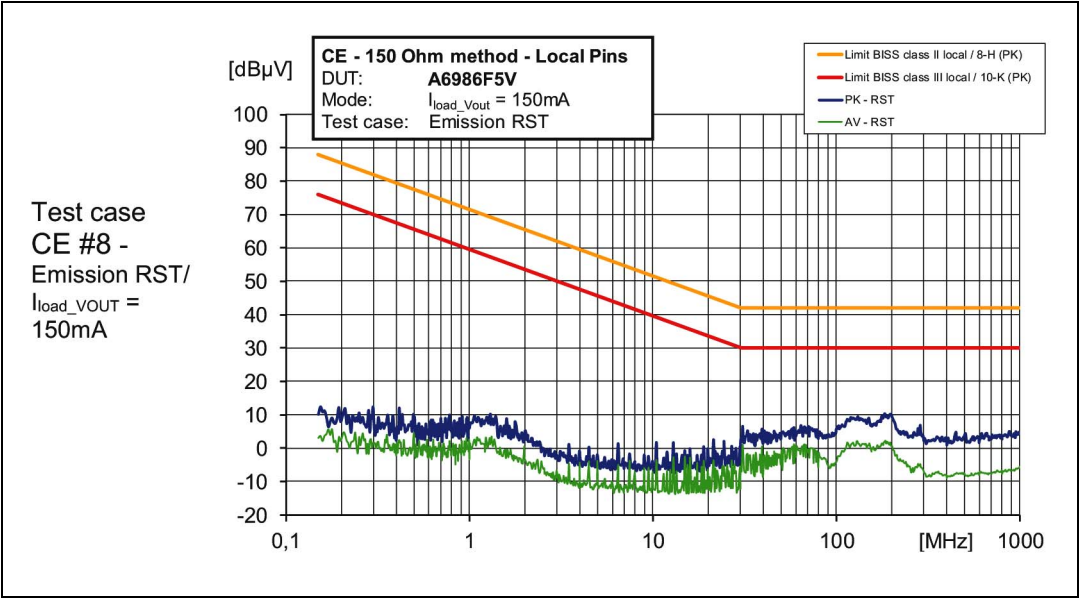
Figure 70. CE 150R at RST test point (see Figure 64 ) at 10% I LOAD
