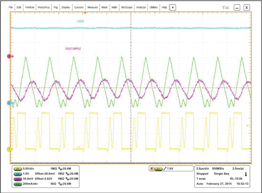
Figure 24. LCM operation over loading condition (part 4 - DCM)
