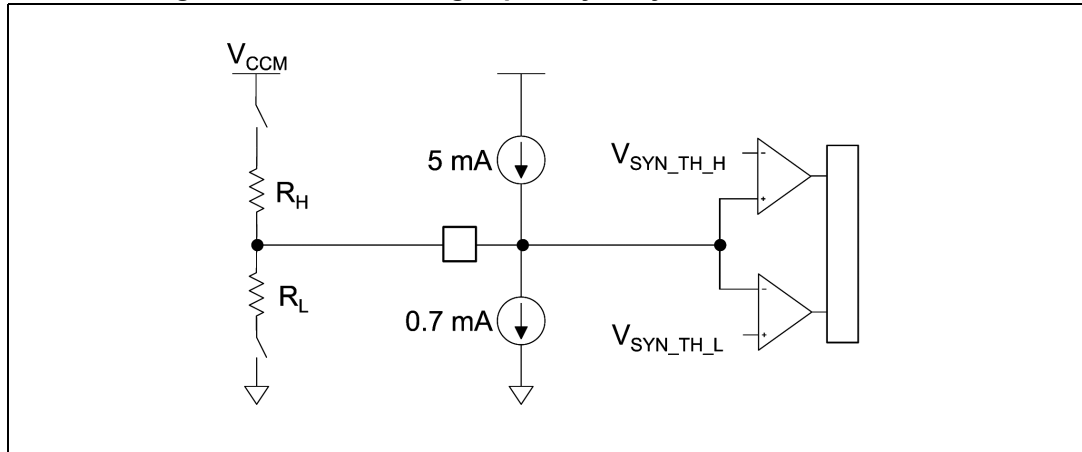
Figure 50. Master driving capability to synchronize the A6986F
