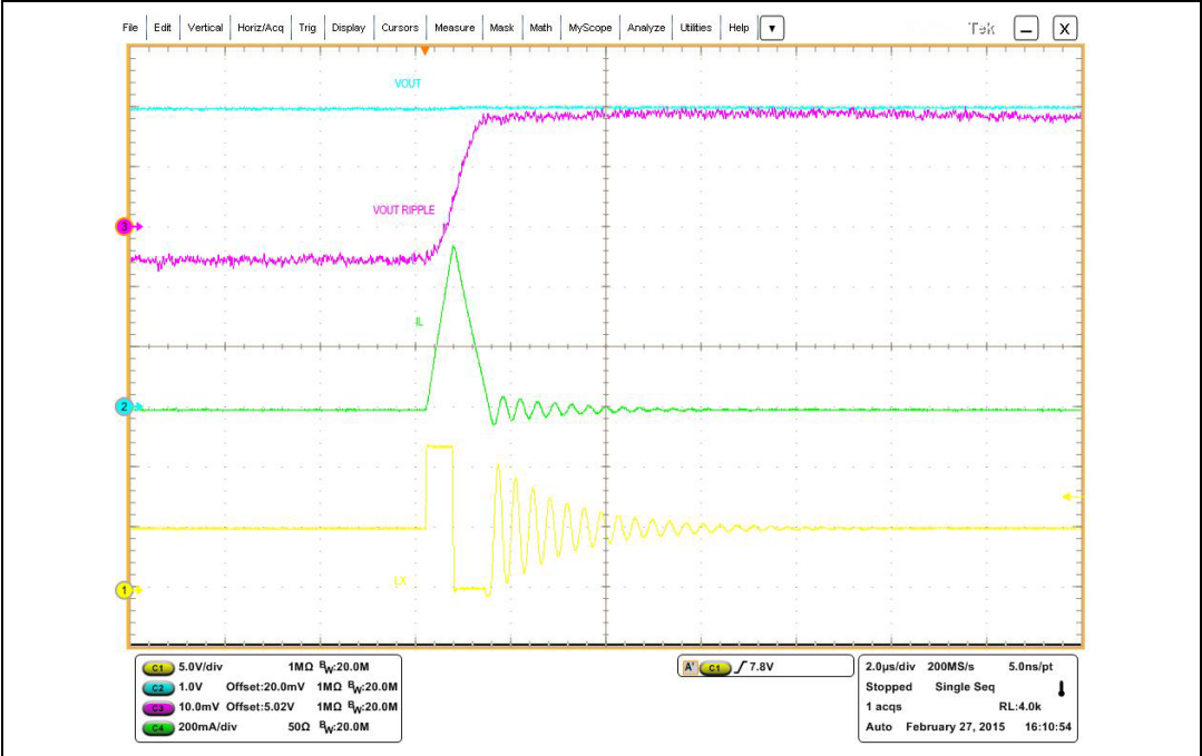
Figure 19. LCM operation with ISKIP_H = 400\text{ mA typ.} at zero load
