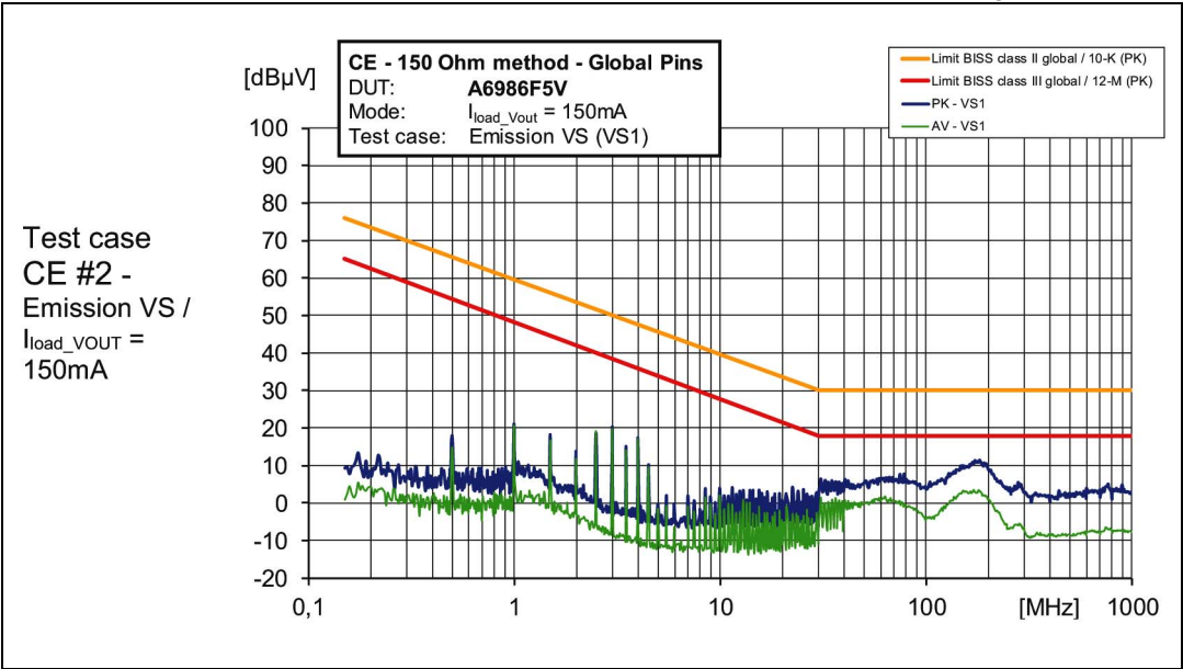
Figure 66. CE 150R at VS1 test point (see Figure 64 ) at 10% I LOAD
