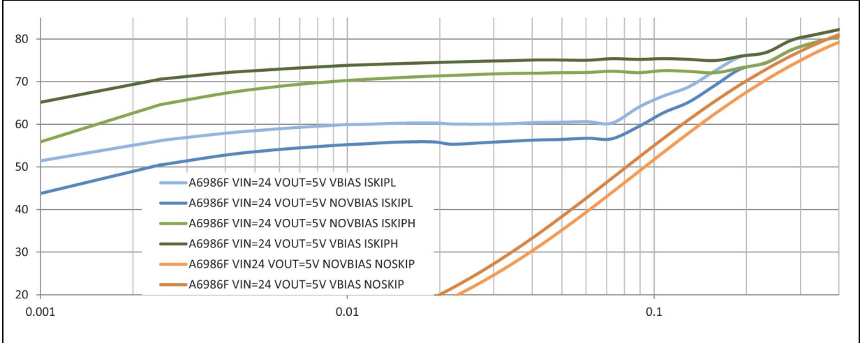
Figure 63. Efficiency curves: V_{IN} = 24\text{ V} - V_{OUT} = 5\text{ V} - f_{sw} = 500\text{ kHz} (log scale)
