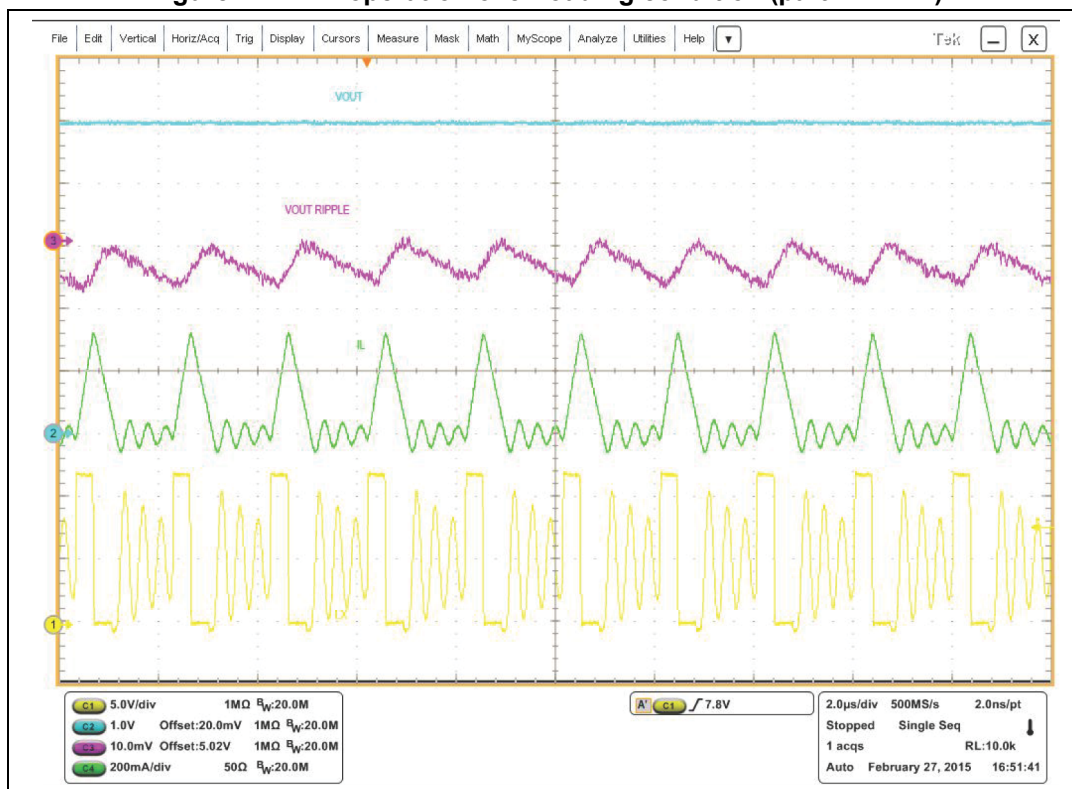
Figure 22. LCM operation over loading condition (part 2 - DCM)
