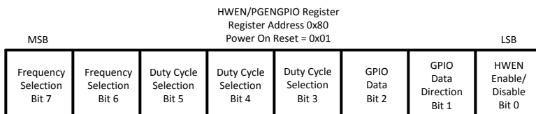
Figure 45. HPG Register Description
