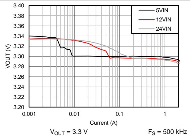
Figure 48. Regulation Curve
