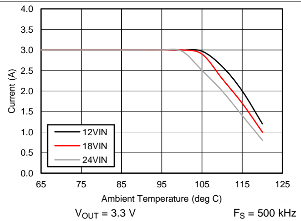
Figure 50. Derating Curve
