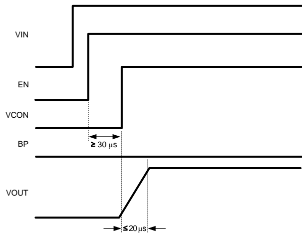
Figure 25. Startup Sequence and Conditions
