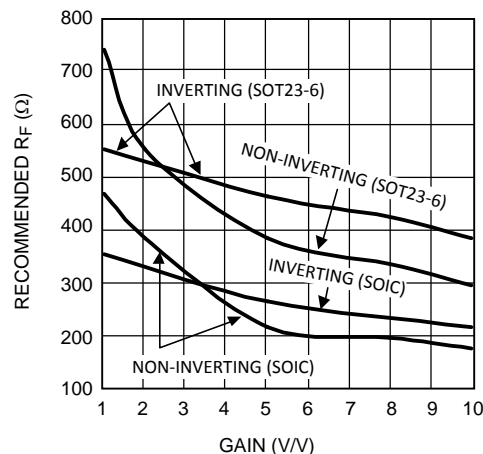
Figure 27. Recommended R_F vs. Gain
