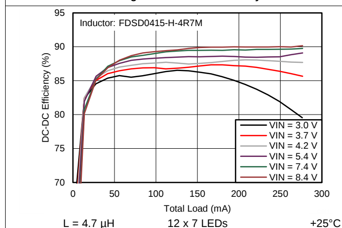
Figure 12. Boost Efficiency
