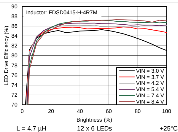
Figure 11. LED Drive Efficiency
