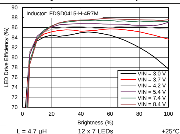
Figure 13. LED Drive Efficiency
