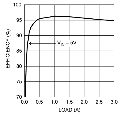
Figure 24. Efficiency
