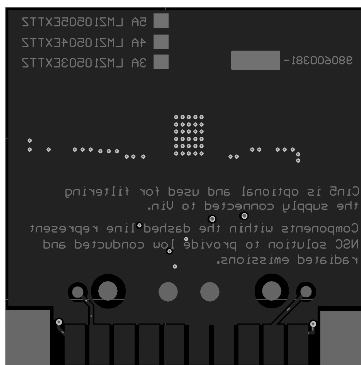
Figure 34. Bottom Copper
