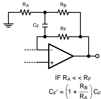
Figure 55. Modified Transimpedance Amplifier
