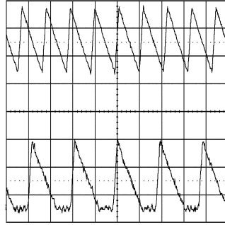
Figure 35. CCM and DCM Operating Modes V_{IN} = 24 \text{ V} , V_O = 3.3 \text{ V} , I_O = 2 \text{ A} / 0.32 \text{ A} 2 \mu s/div
