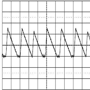
Figure 36. Transition Mode Operation V_{IN} = 24 \text{ V} , V_O = 3.3 \text{ V} , I_O = 0.35 \text{ A} 2 \mu s/div
