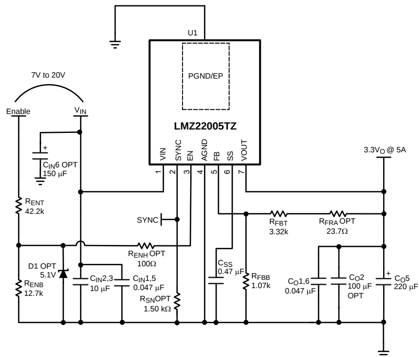
Figure 46. Typical Application Schematic
