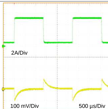
Figure 40. Output Ripple
