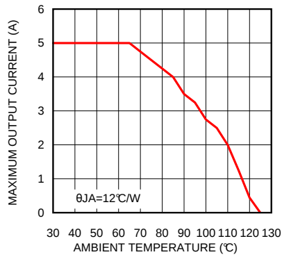
Figure 37. Thermal Derating
