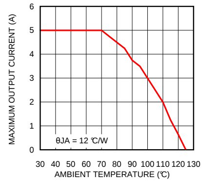
Figure 38. Thermal Derating
